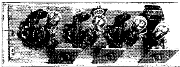
FIGURE 6. THE SCREEN-GRID AMPLIFIER WITH THE SHIELDS REMOVED
