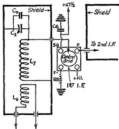
FIGURE 13. THE WIRING OF THE FIRST INTERMEDIATE-FREQUENCY STAGE
